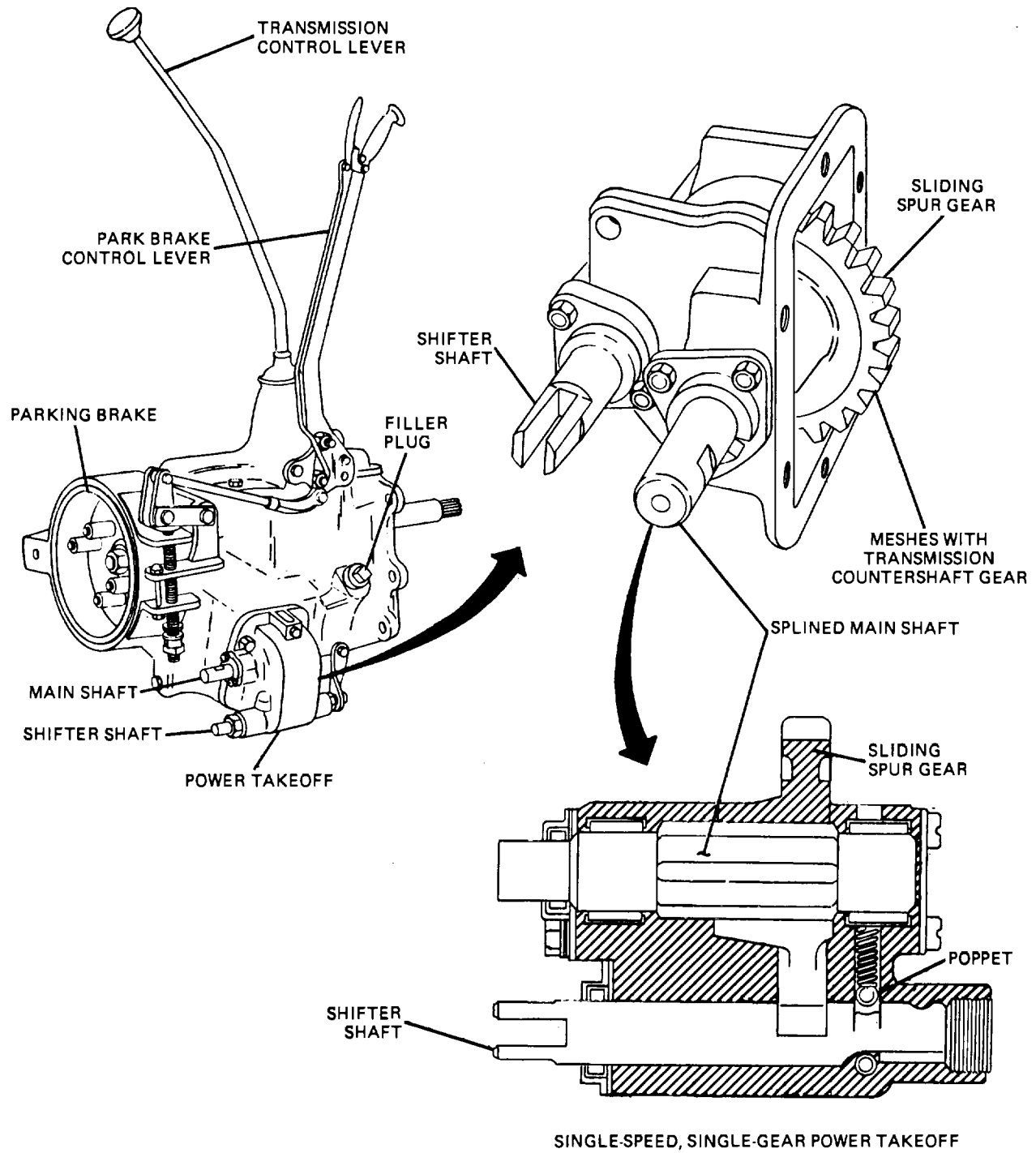
Figure 19-1. Power Takeoff.
