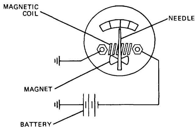
Figure 17-2. Ammeter Operation
