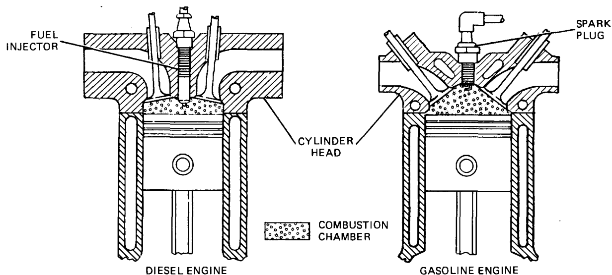
Figure 3-6. Combustion Chambers.
