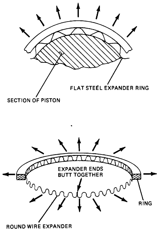
Figure 3-28. 3-8. Connecting Rods.
