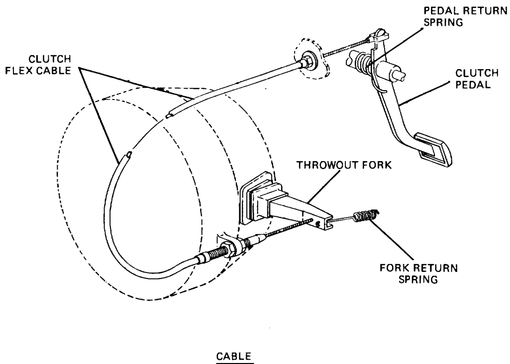
Figure 21-8. Mechanical Operating Systems.
