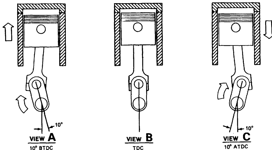
Figure 2-51. Ignition Timing
