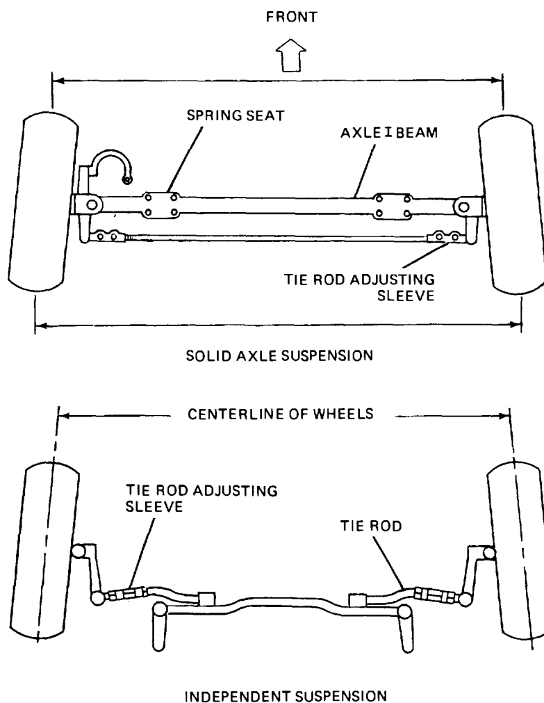
Figure 33-24. Toe-in
