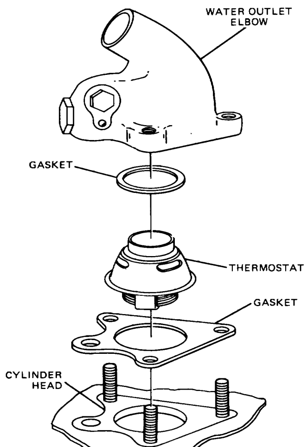
Figure 9-7. Bellows Type Thermostat
