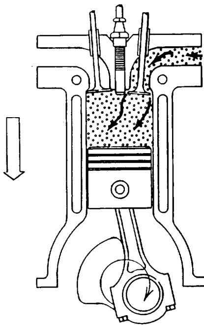
A. INTAKE STROKE
