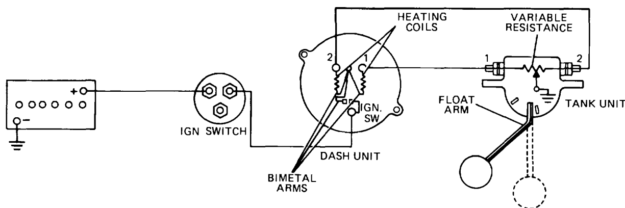
Figure 17-8. Thermostatic Fuel Gage: Differential Type
