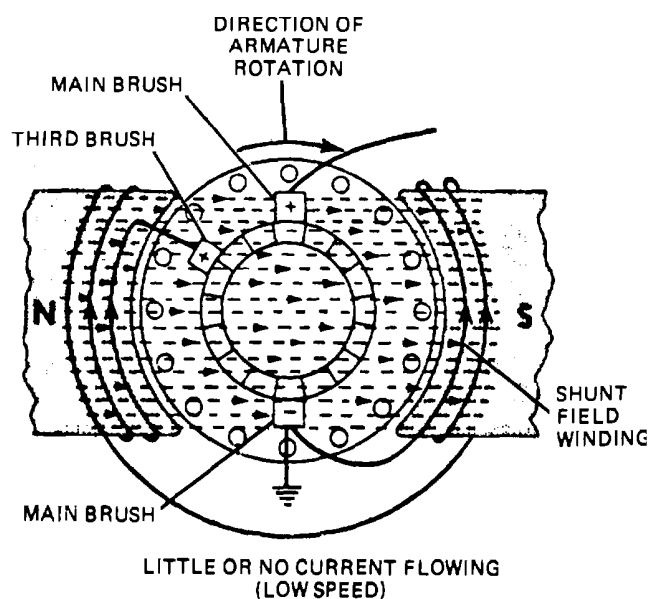
Figure 13-13. Third-Brush Regulation.
