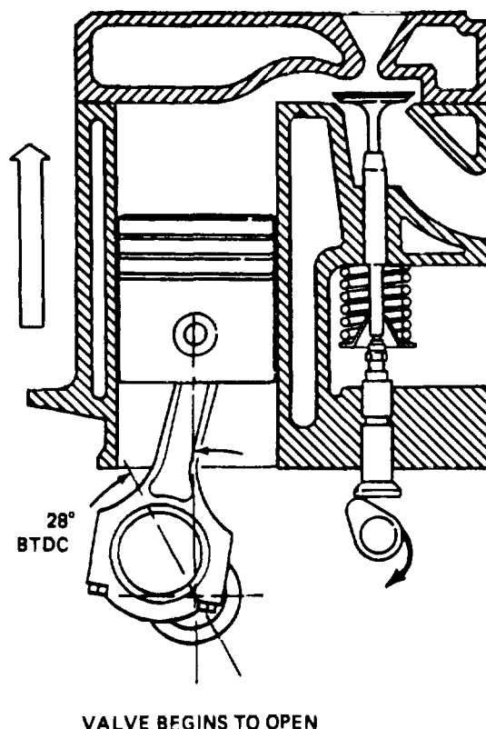
Figure 2-53. Opening and Closing Points of the Valve.
