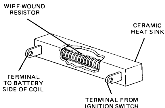
Figure 15-10. Ballast Resistor
