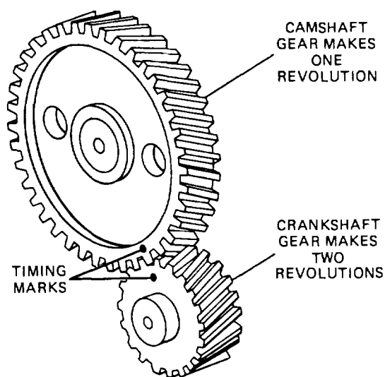
Figure 2-10. Timing Gears
