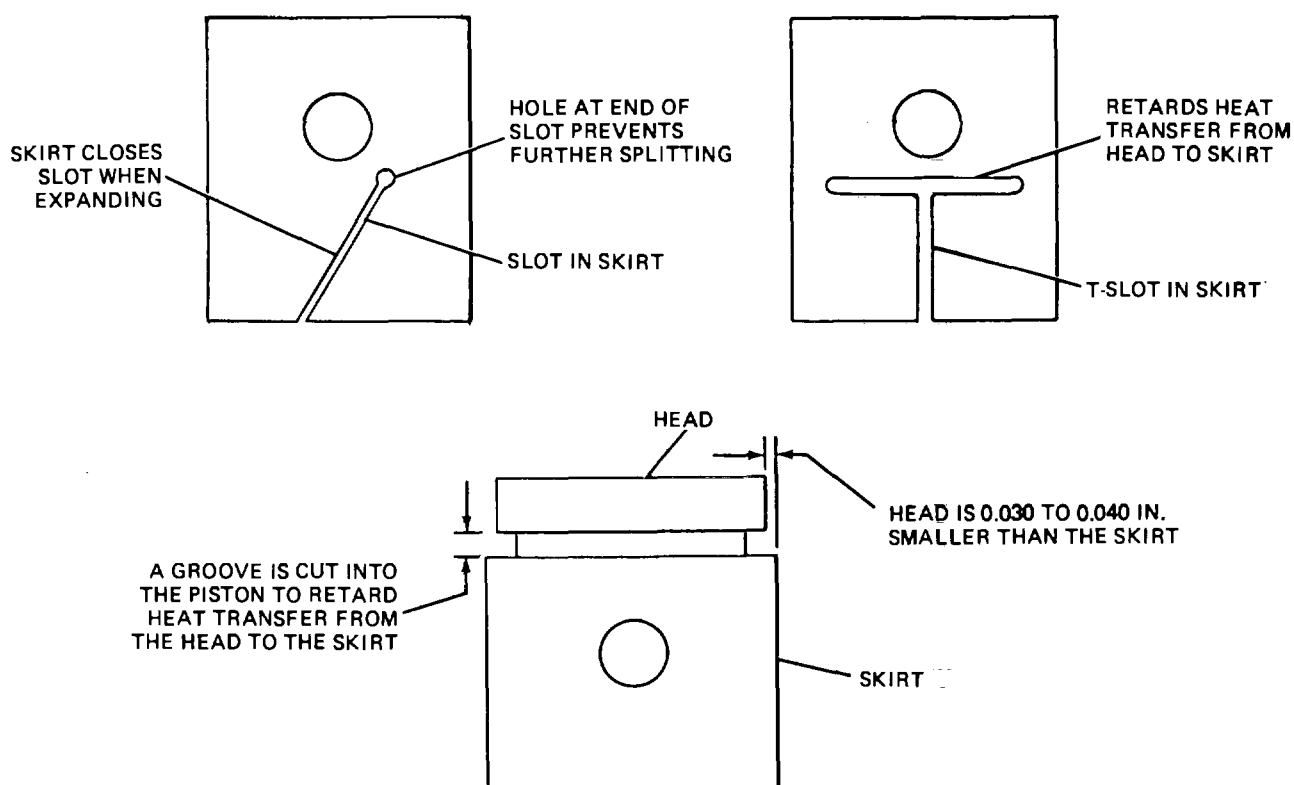
Figure 3-13. Controlling Piston Expansion.
