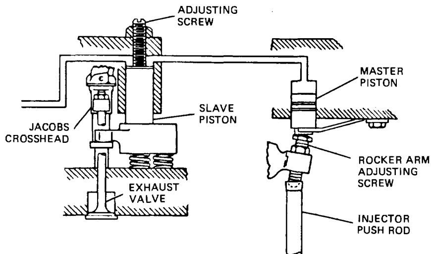
Figure 5-31. Jacobs Engine Break
