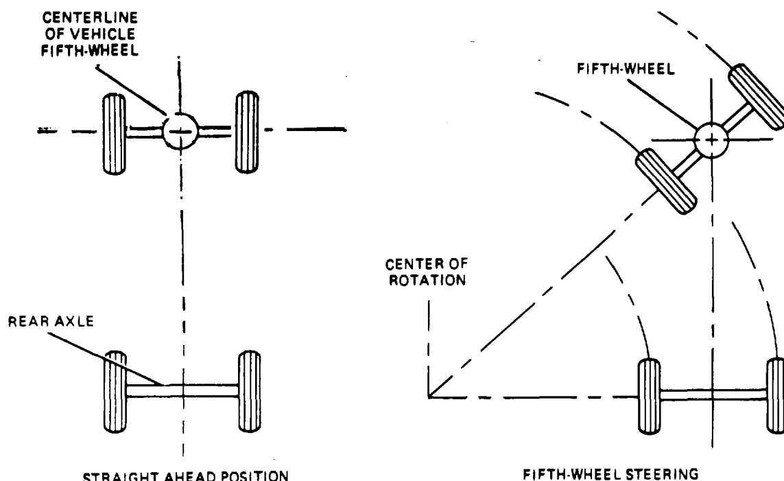
Figure 33-2. Fifth-Wheel Steering
