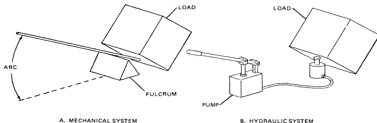
Figure 20-3. Mechanical Advantage.
