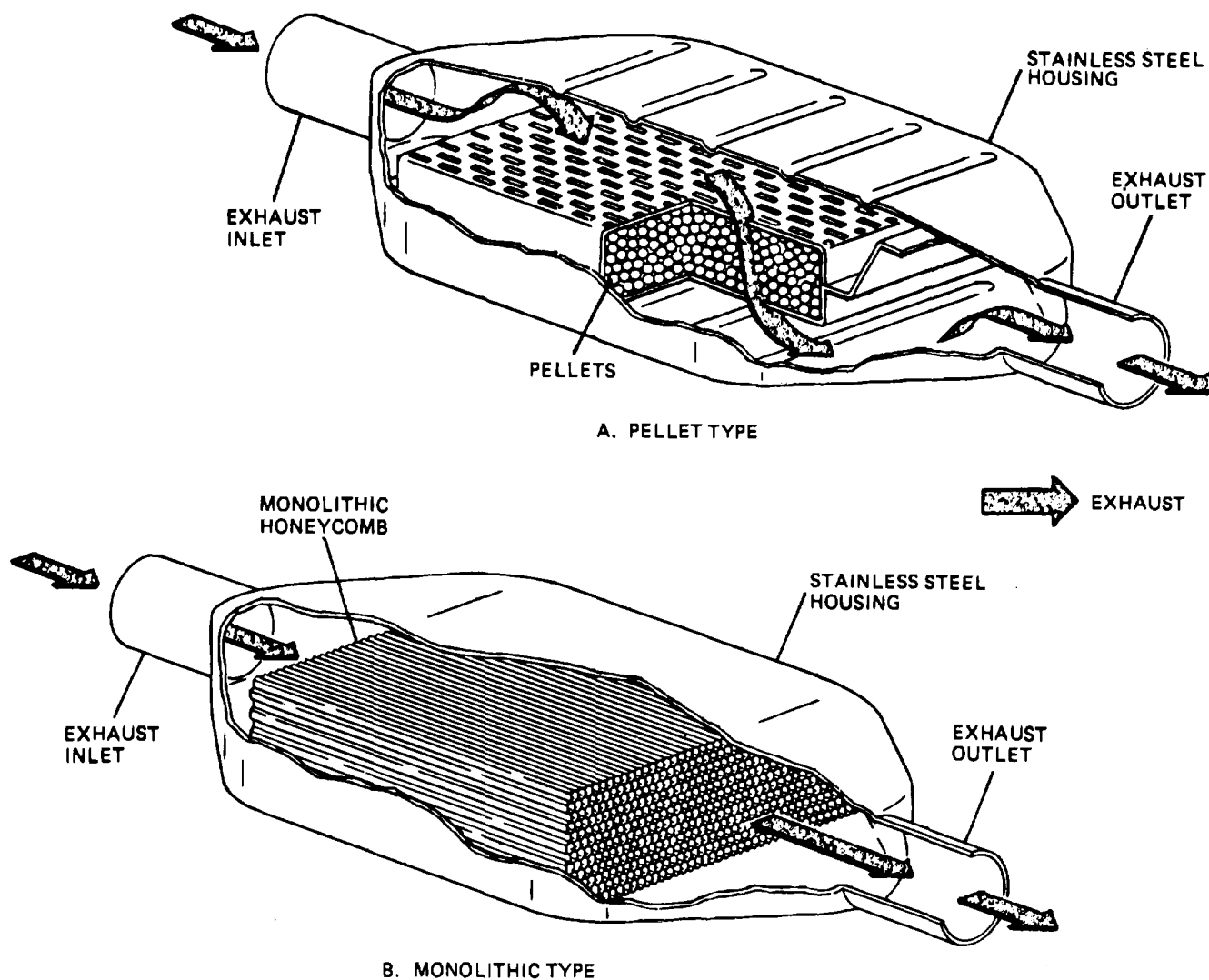
Figure 7-8. Catalytic Converter
