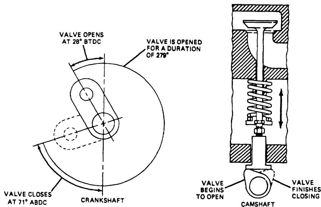
Figure 2-54. Valve Opening Duration
