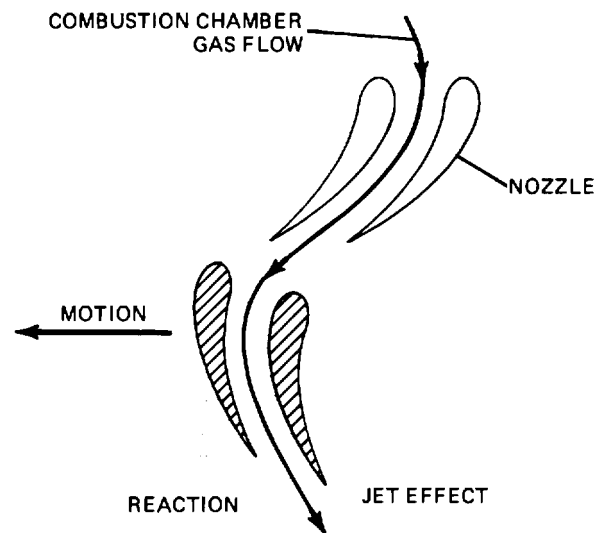
Figure 10-15. Reaction Turbine
