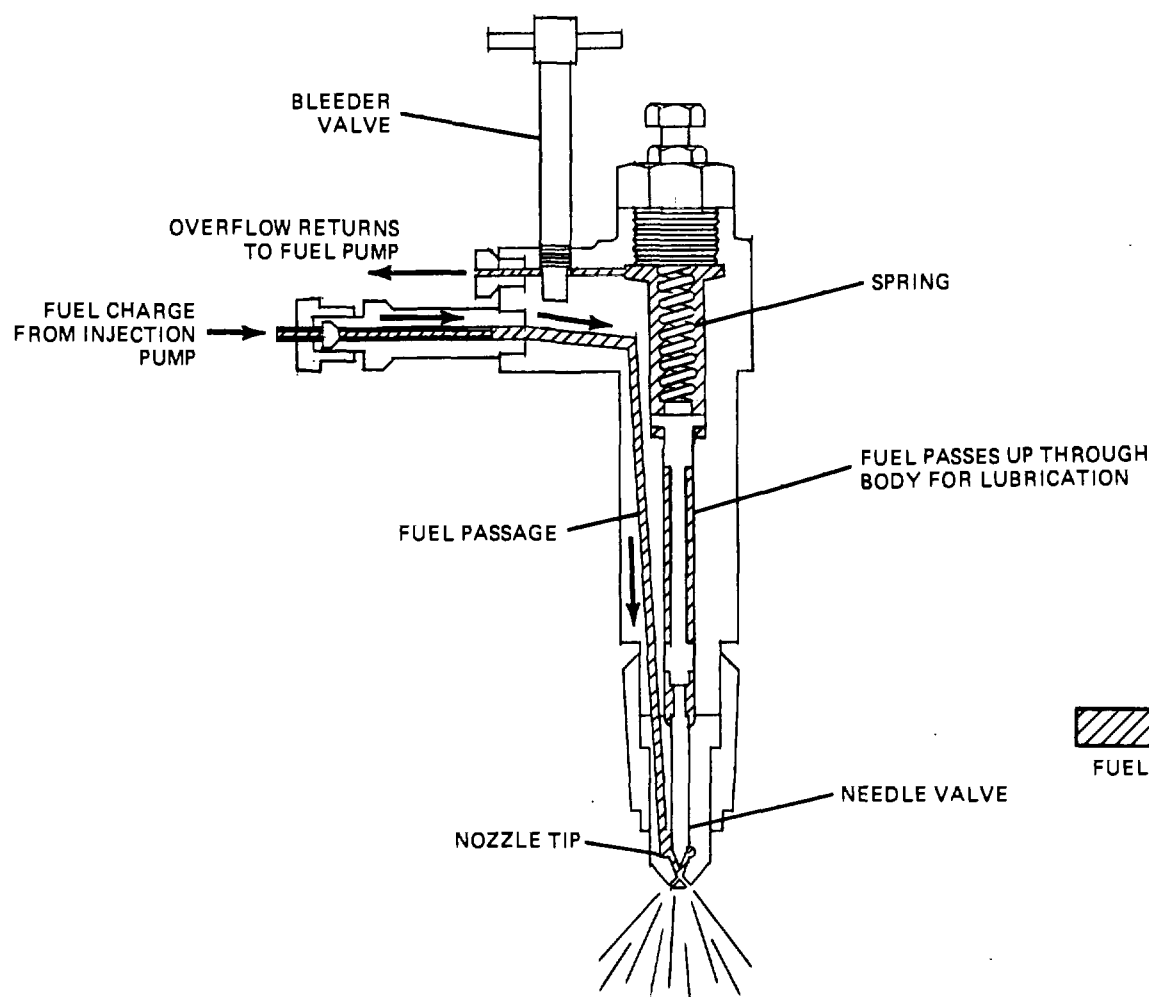
Figure 5-8. Multiple Unit Injector.
