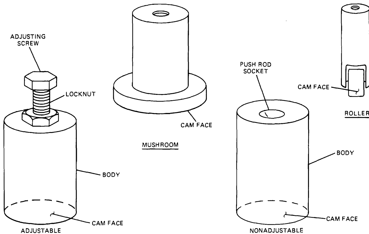
Figure 3-55. Mechanical Tappets.
