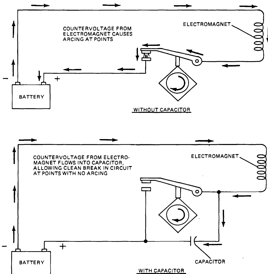
Figure 15-2. Capacitor Action.
