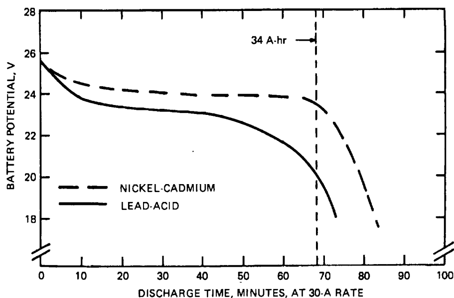
Figure 12-7. Comparison of Discharge Characteristics.
