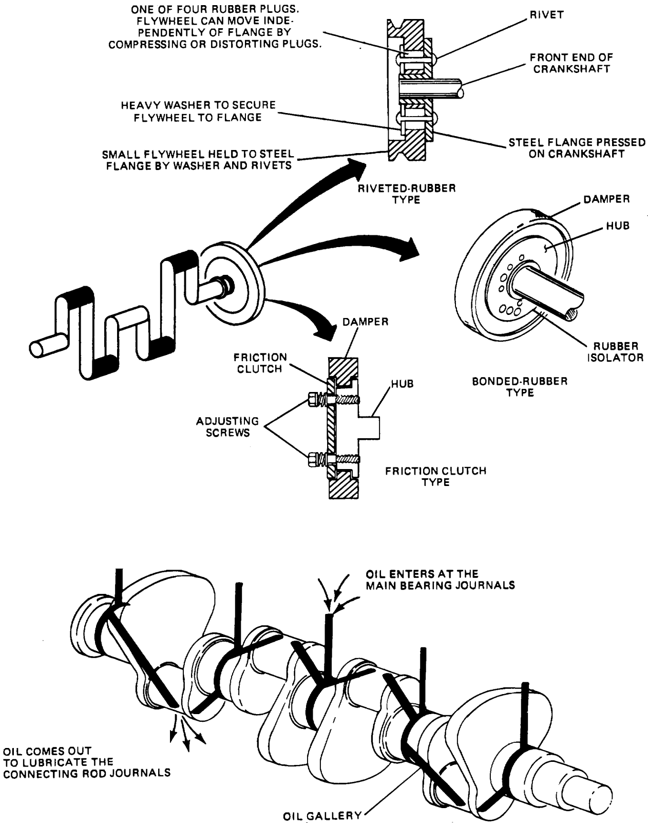
Figure 3-37. Figure 3-38. Crankshaft Lubrication Passages. 3-23
