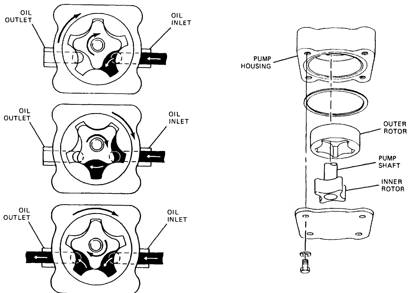
Figure 20-5. Rotary Pumps.
