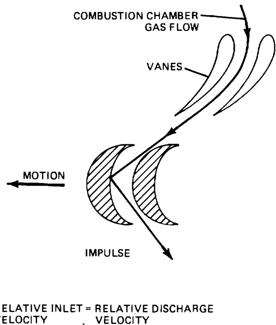
Figure 10-14. Impulse Turbine
