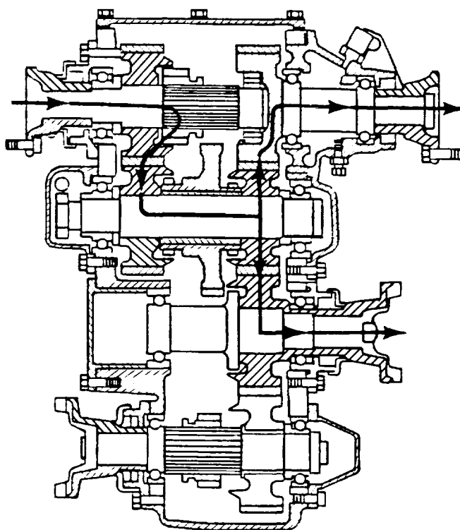
HIGH RANGE - REAR AXLES ONLY DRIVING
