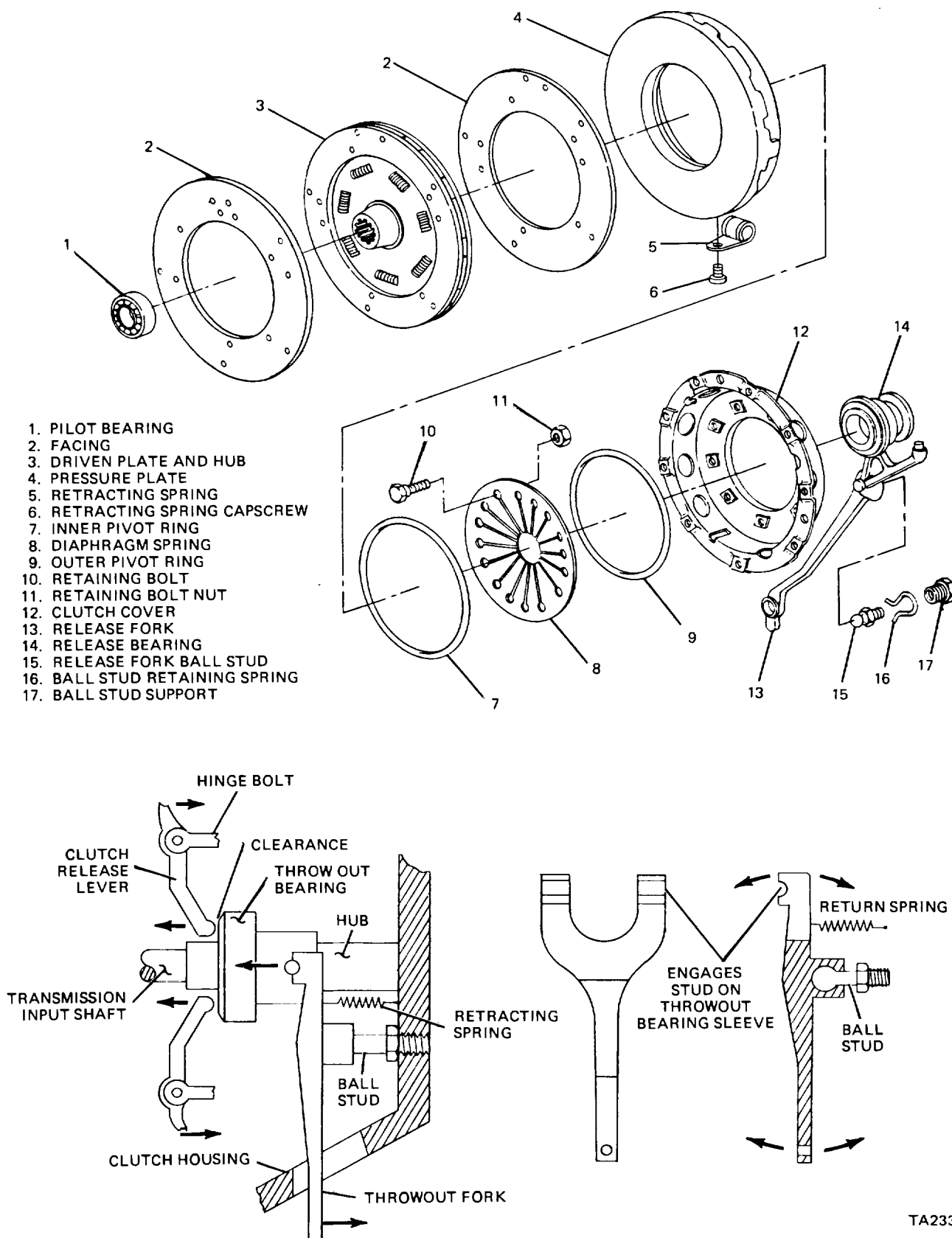
Figure 21-6. & Figure 21-7. Clutch Activation.
