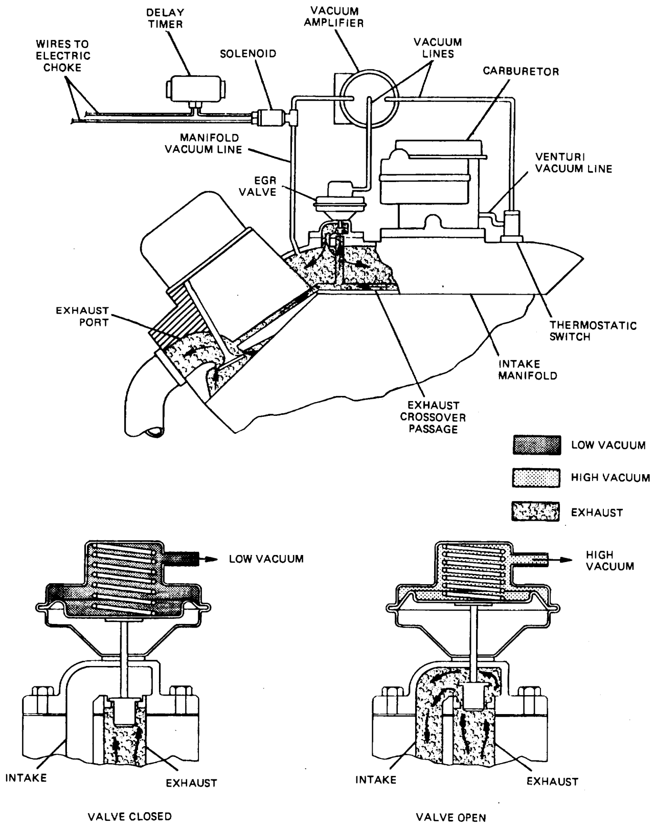
Figure 7-11. EGR System.
