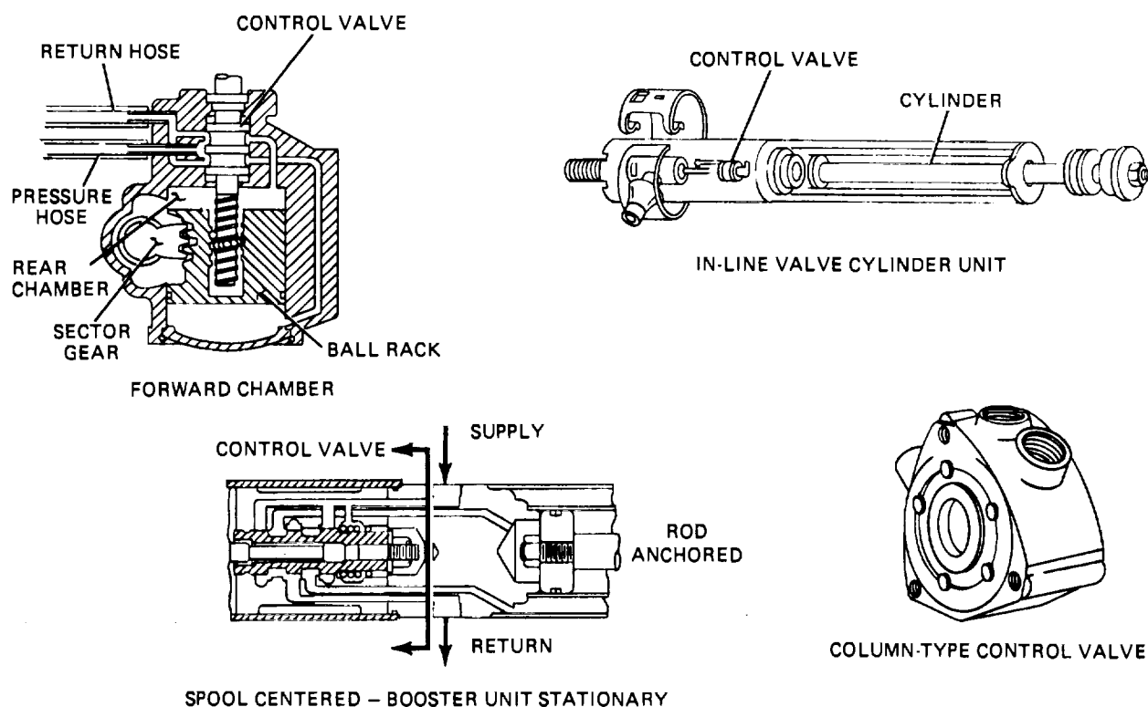
Figure 33-13. Control Valve
