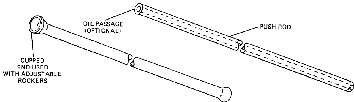
Figure 3-58. Push Rod.
