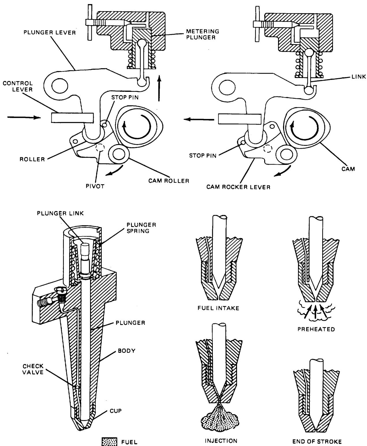
Figure 5-12. & Figure 5-13. Distributor-Type Unit Injectors.
