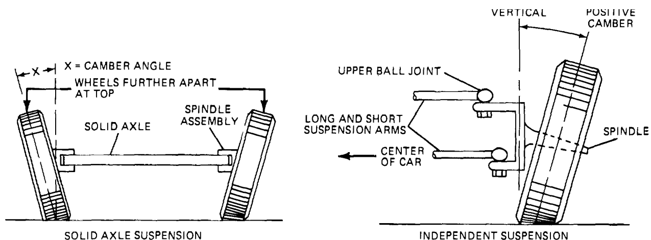
Figure 33-22. Kingpin inclination
