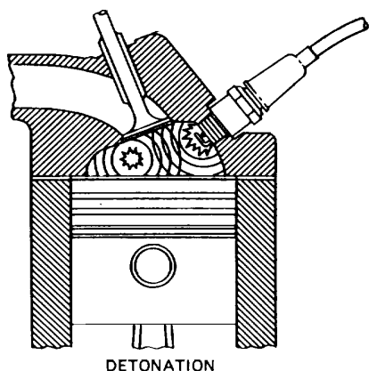
Figure 4-77. Detonation.
