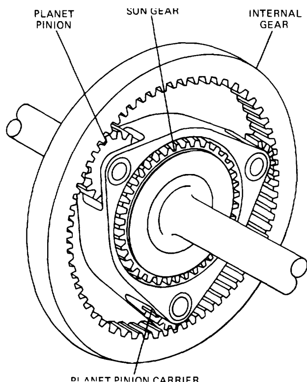
Figure 19-6. Planetary Gear System
