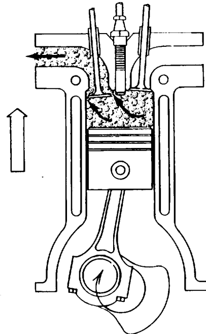
D. EXHAUST STROKE
