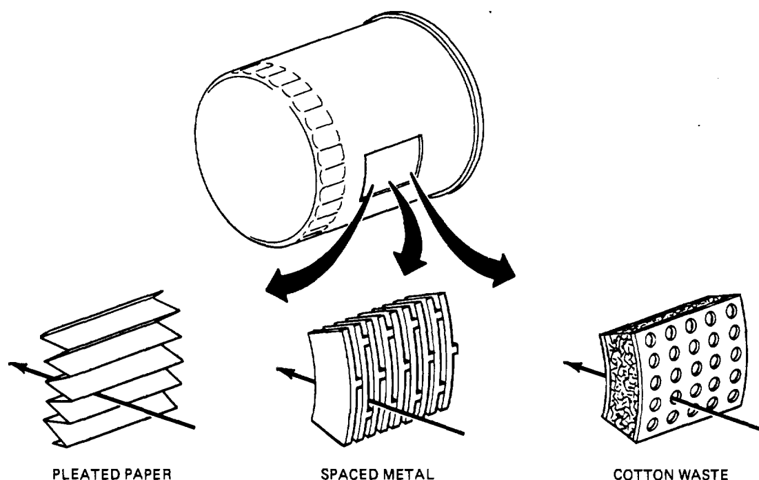
Figure 8-8. Oil Filtering Mediums
