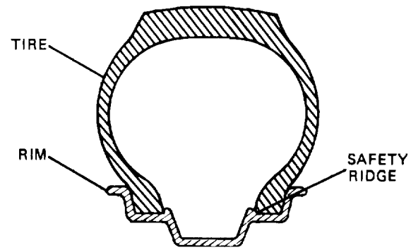
Figure 32-6. Safety Rim
