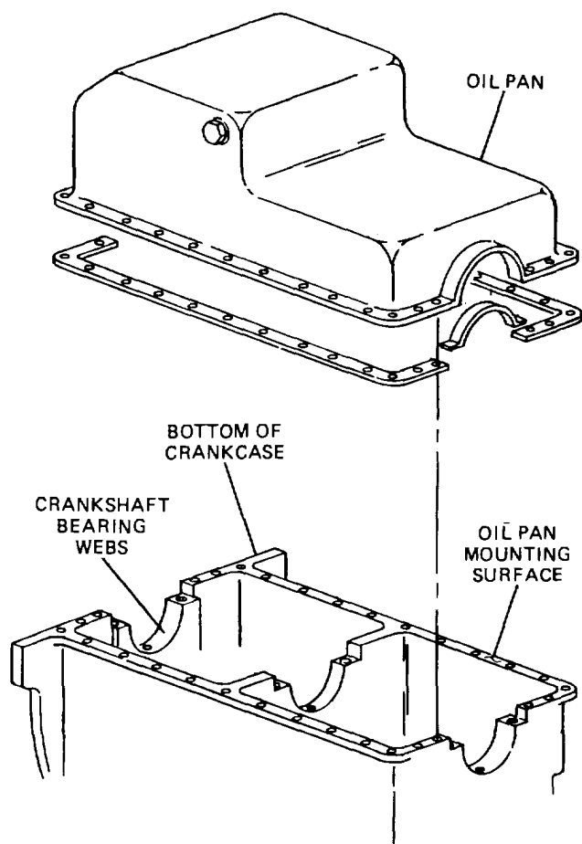
Figure 3-4. Engine Crankcase.
