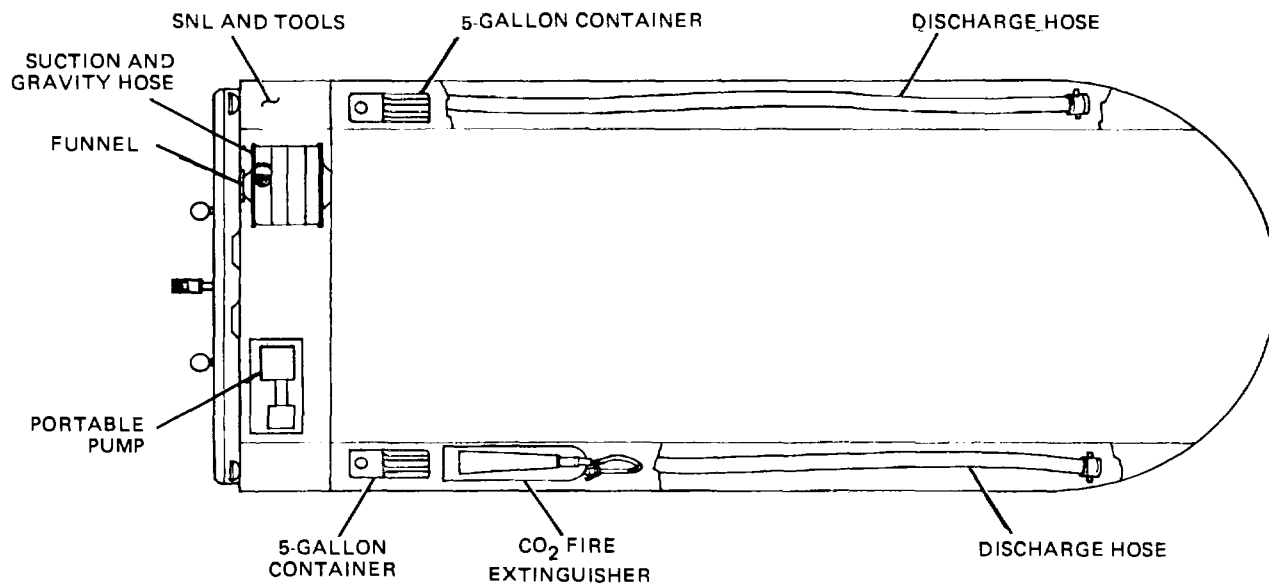
Figure 36-10. Location of Portable Pump and Hose in Tank Semitrailer.
