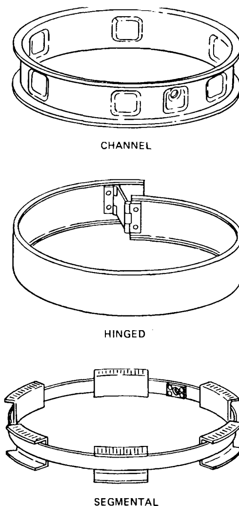
Figure 32-8. Bead Locks.
